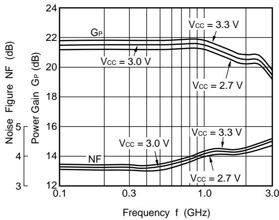
NOISE FIGURE, POWER GAIN vs. FREQUENCY
