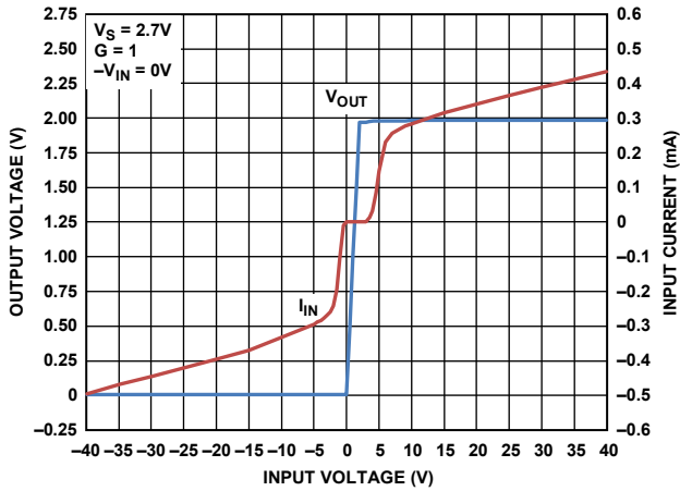
Figure 16. Input Overvoltage Performance, Single Supply, V_S = 2.7V , G = 1
