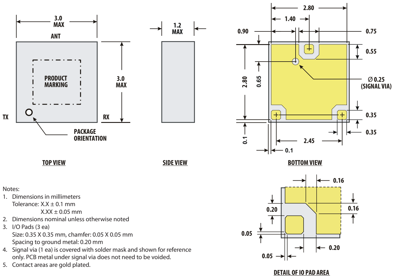
Figure 17. Package Outline Drawing.
