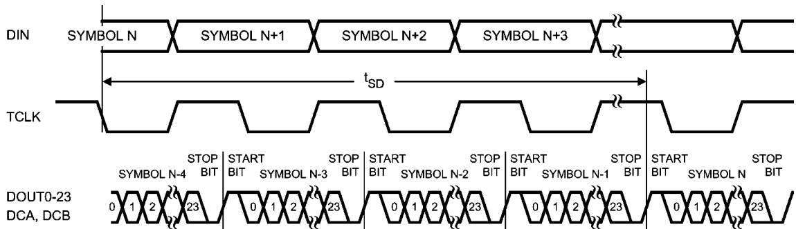
FIGURE 8. Serializer Delay
