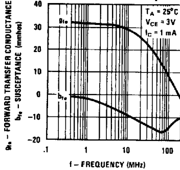
Typical Forward Transfer Admittance vs Frequency
