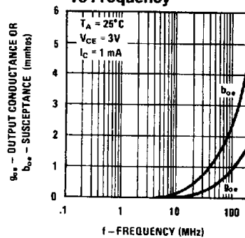
Typical Output Admittance vs Frequency
