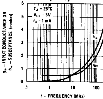
Typical Input Admittance vs Frequency
