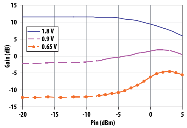
Figure 10. Gain vs. Pin at 6 GHz
