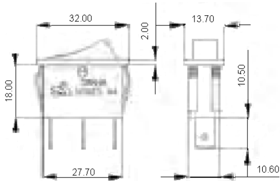
Dimensions: Millimetres
