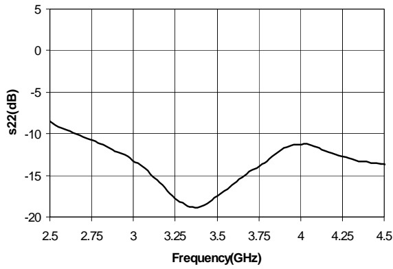
3GHz Tune Output Return Loss +25c
