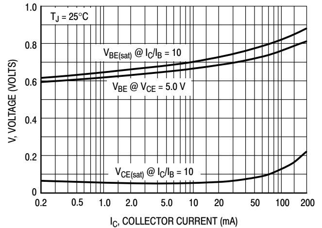
Figure 14. "ON" Voltages
