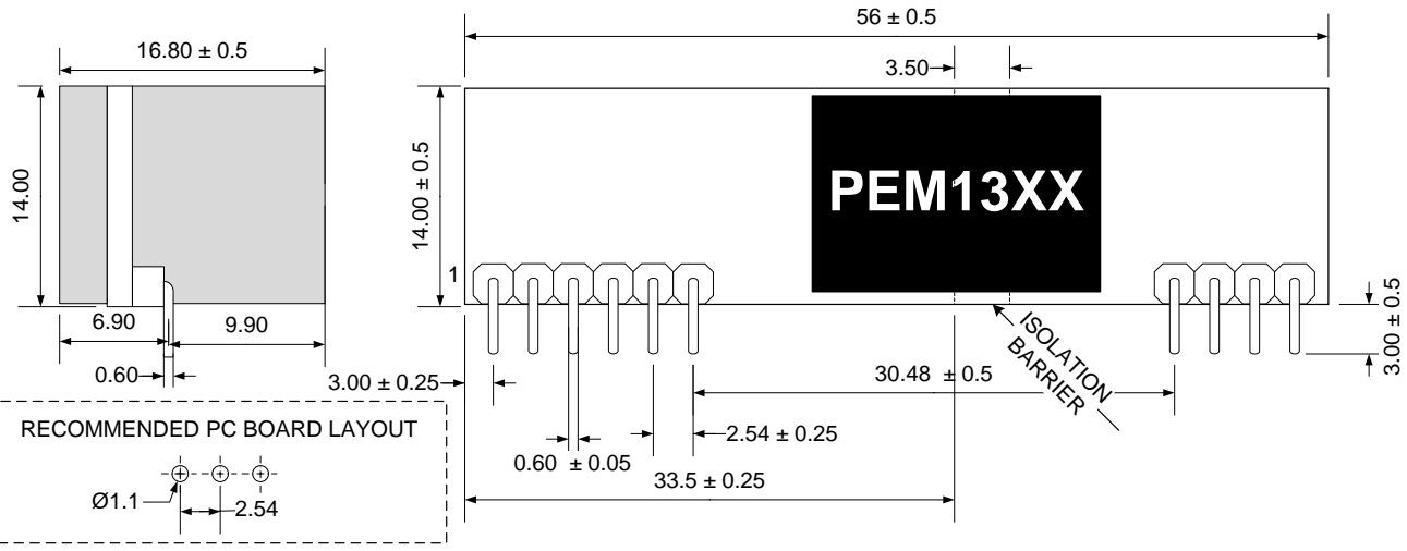
Figure 6 – PHYSICAL PACKAGE
