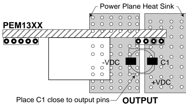
Figure 8 – Power Plane Heat Sink
