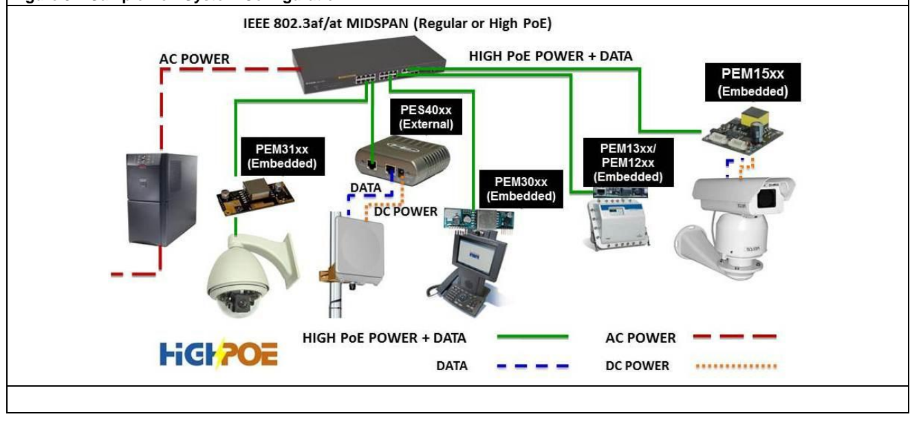
Figure 9 – Sample PoE System Configuration
