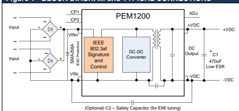
Figure 1 - BLOCK DIAGRAM and TYPICAL CONNECTIONS
