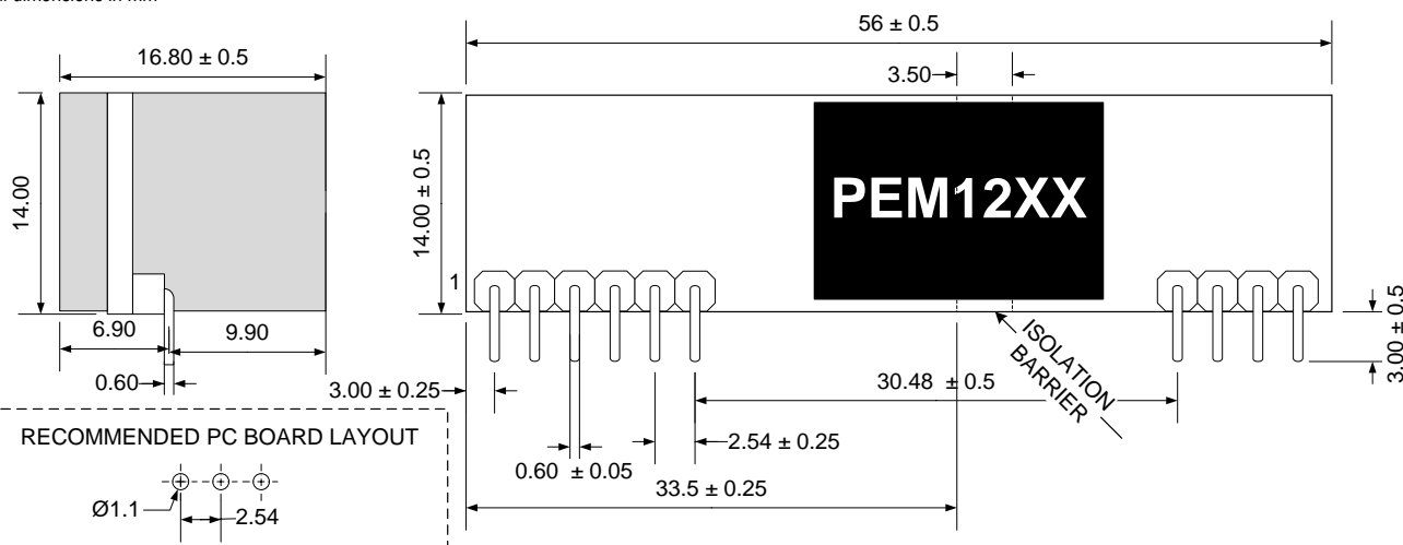
Figure 6 – PHYSICAL PACKAGE
