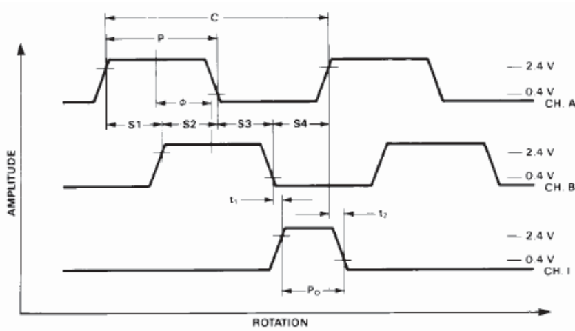
Figure 2. Output waveforms
