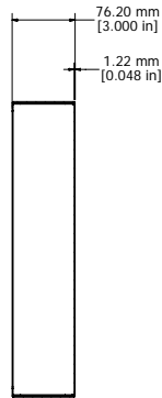
SECTION PP-PP
