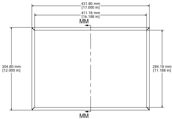
1441-34 OR 1441-34BK3 - VIEW FROM TOP (SOLD SEPERATELY)
