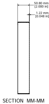
SECTION MM-MM
