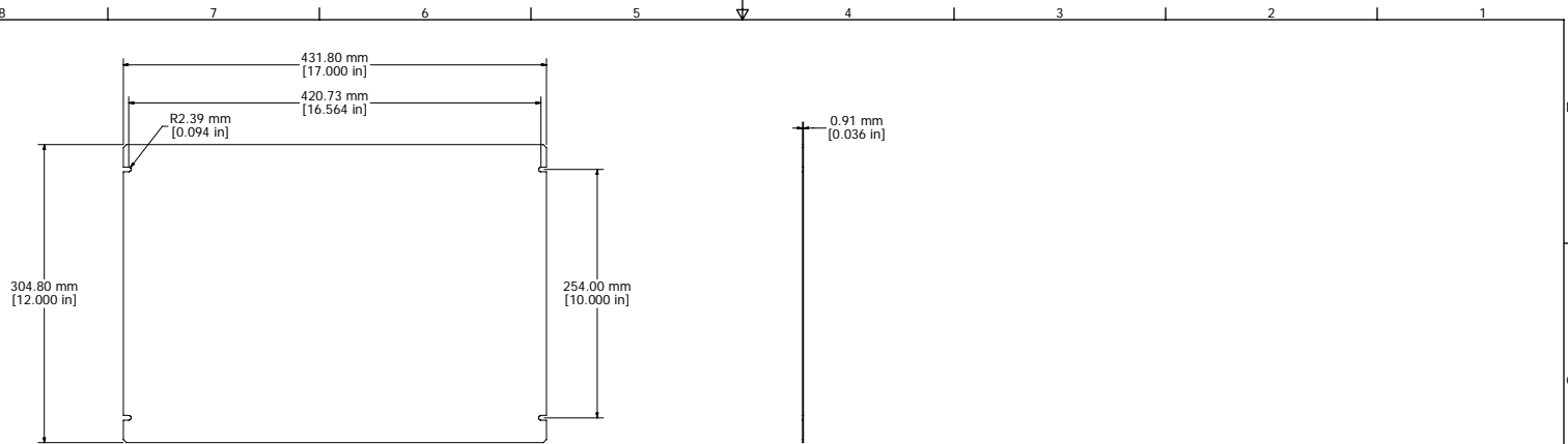
1431-34 OR 1431-34BK3 - VIEW FROM TOP (SOLD SEPERATELY)
