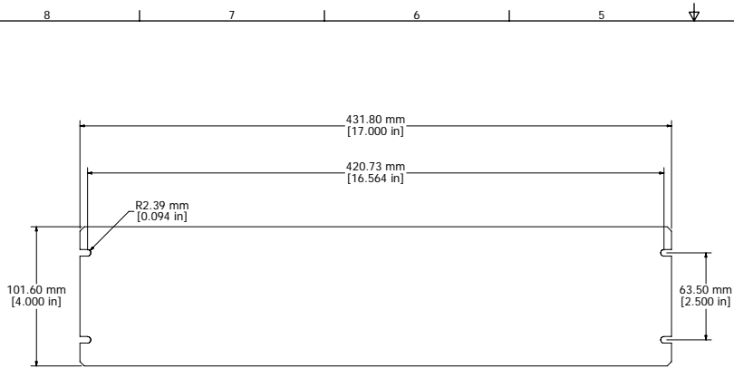
1431-20 OR 1431-20BK3 - VIEW FROM TOP (SOLD SEPERATELY)
