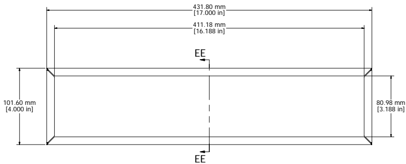
1441-20 OR 1441-20BK3 - VIEW FROM TOP (SOLD SEPERATELY)
