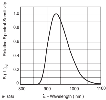
Figure 10. Relative Spectral Sensitivity vs. Wavelength
