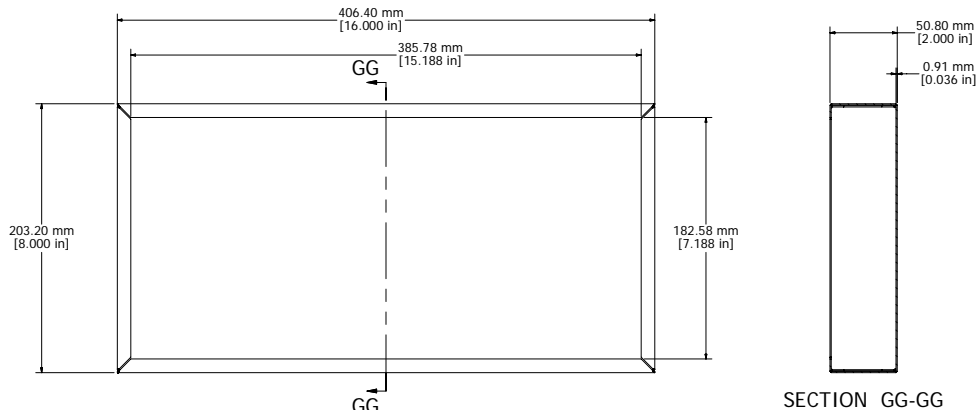
1441-26 OR 1441-26BK3 - VIEW FROM TOP (SOLD SEPERATELY)
