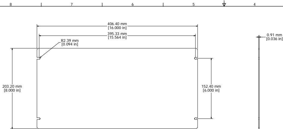
1431-26 OR 1431-26BK3 - VIEW FROM TOP (SOLD SEPERATELY)
