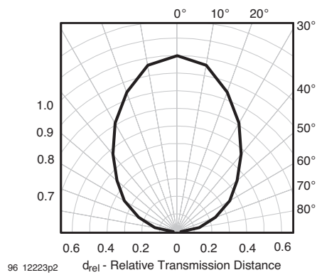
Figure 12. Directivity
