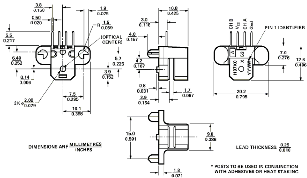
Mounting Option #53 – Standard with Posts (Baseplane Mounting)
