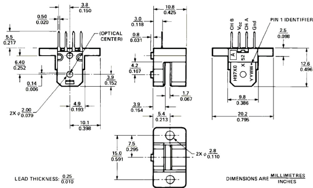
Mounting Option #52 – Backplane (Backplane Mounting)
