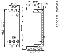
Sealable cover COV.01
