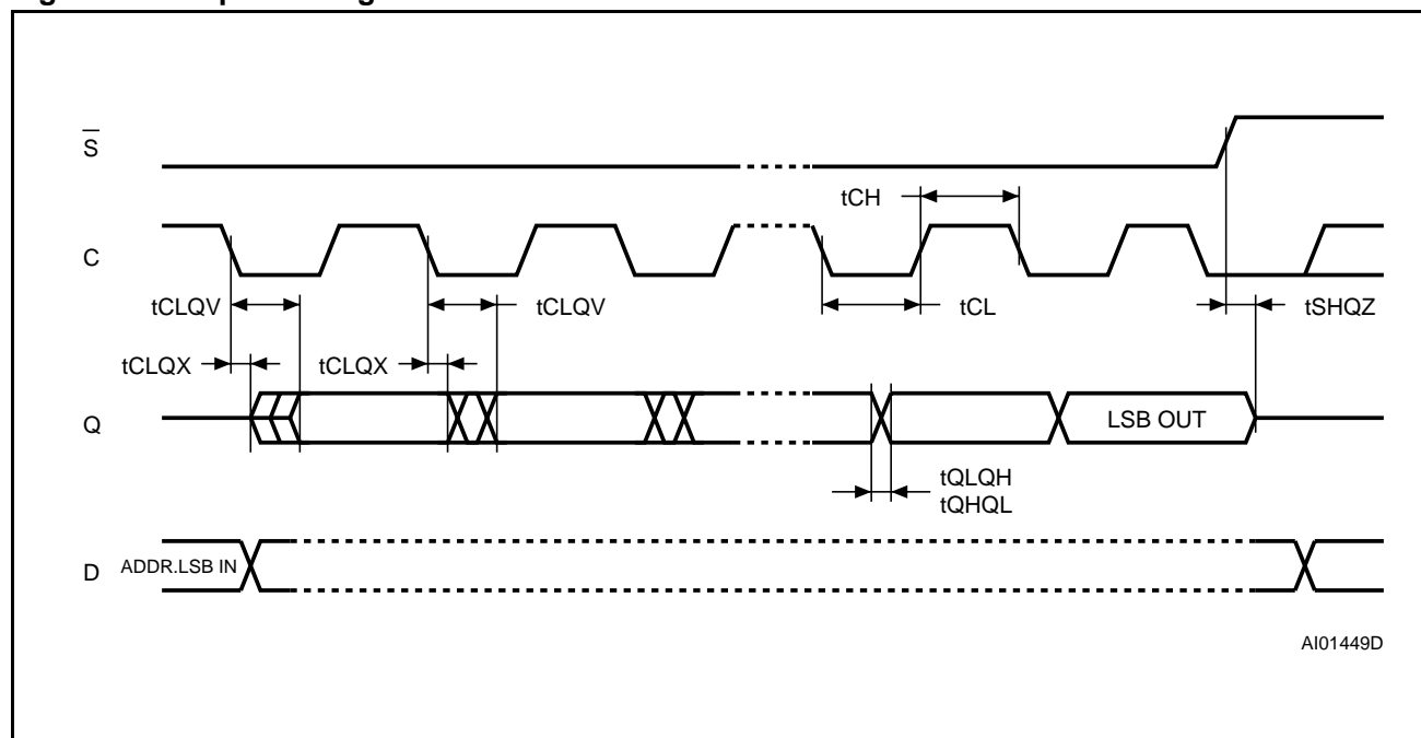
Figure 25. Output Timing
