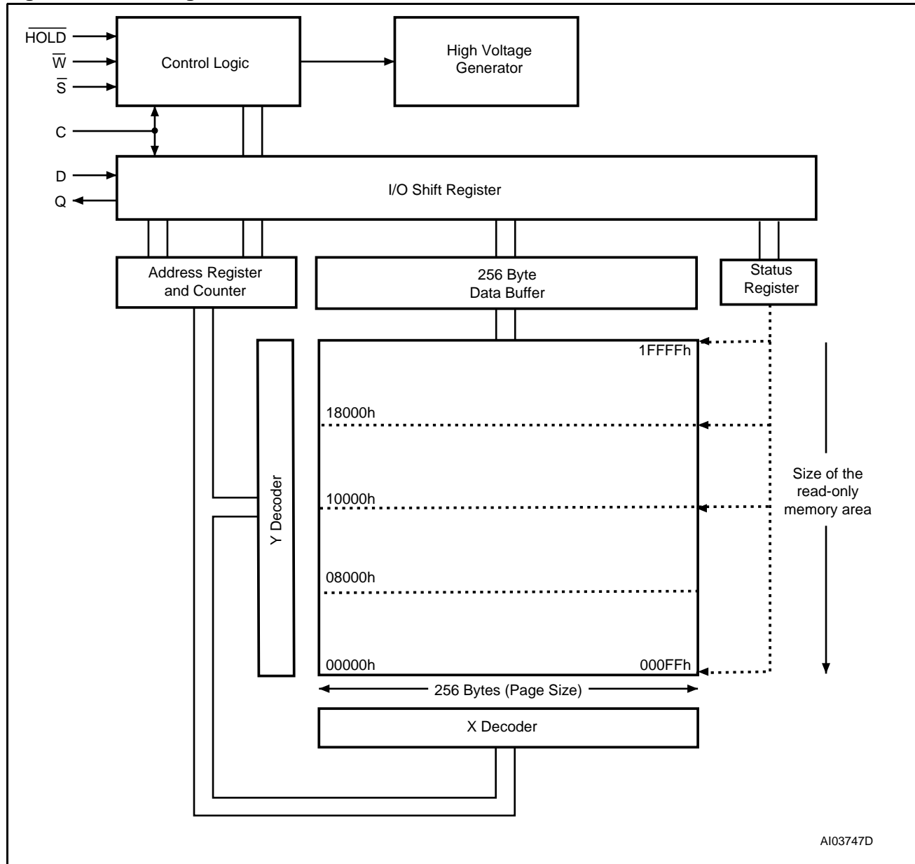
Figure 7. Block Diagram
