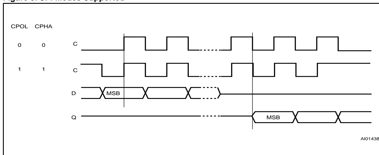
Figure 5. SPI Modes Supported
