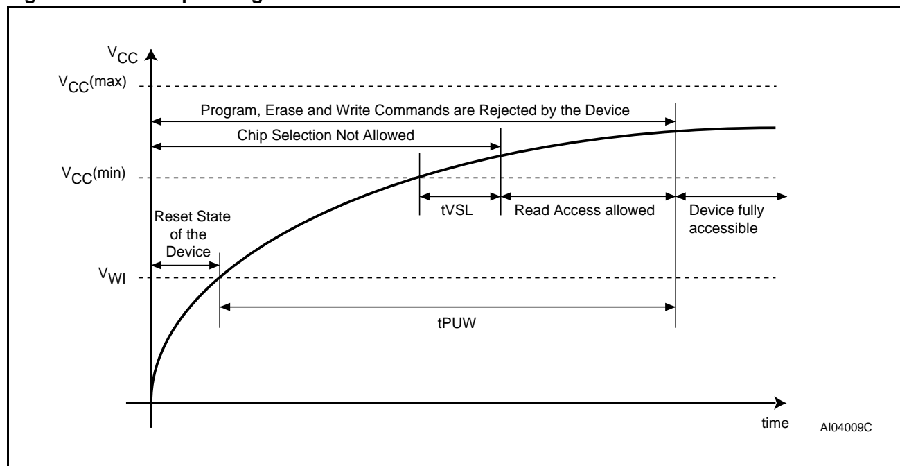
Figure 20. Power-up Timing
