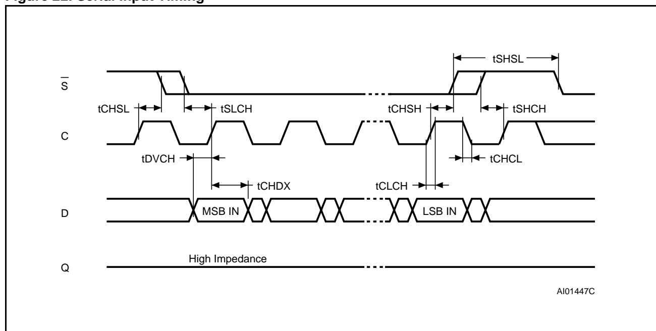
Figure 22. Serial Input Timing
