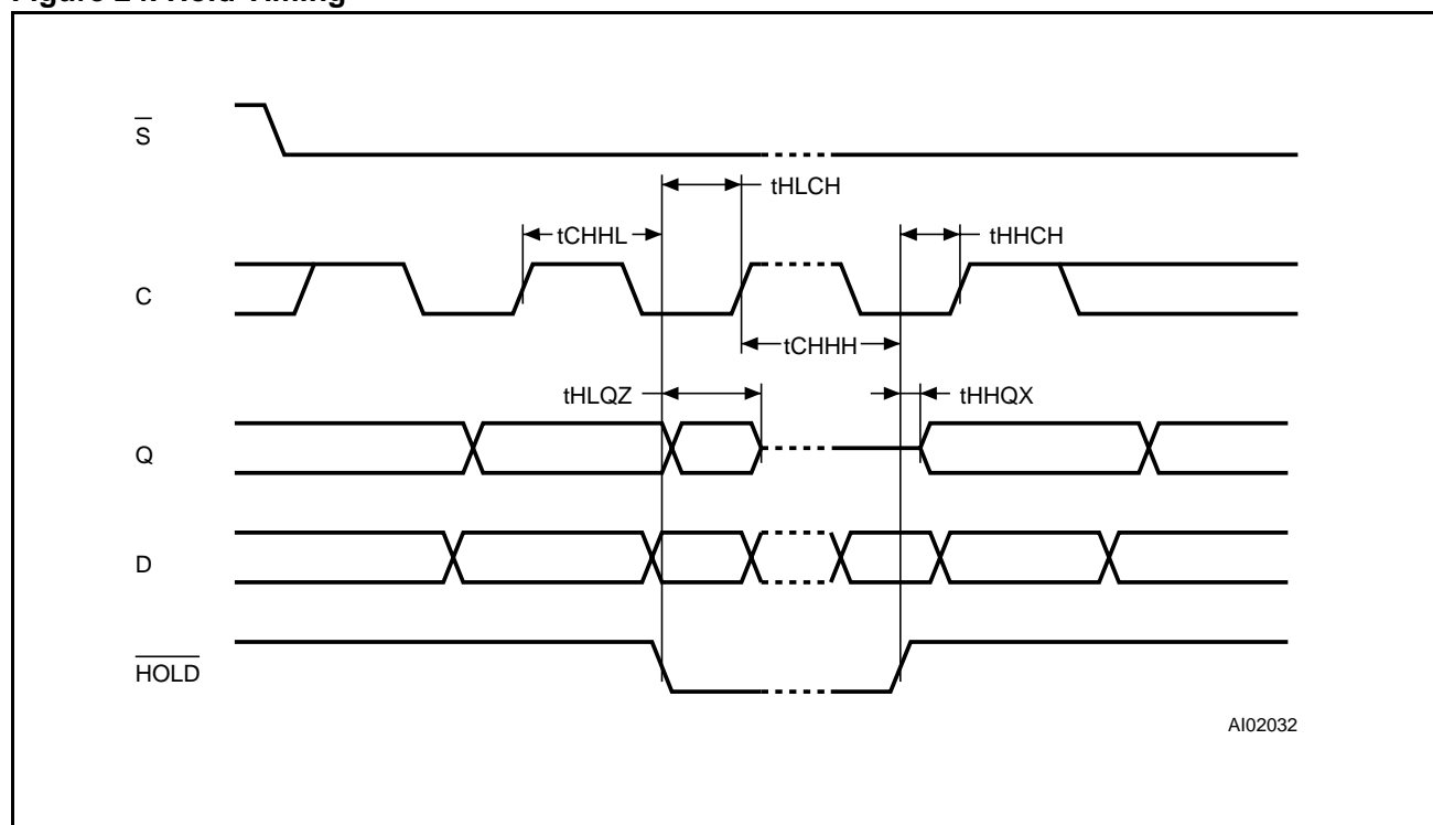
Figure 24. Hold Timing
