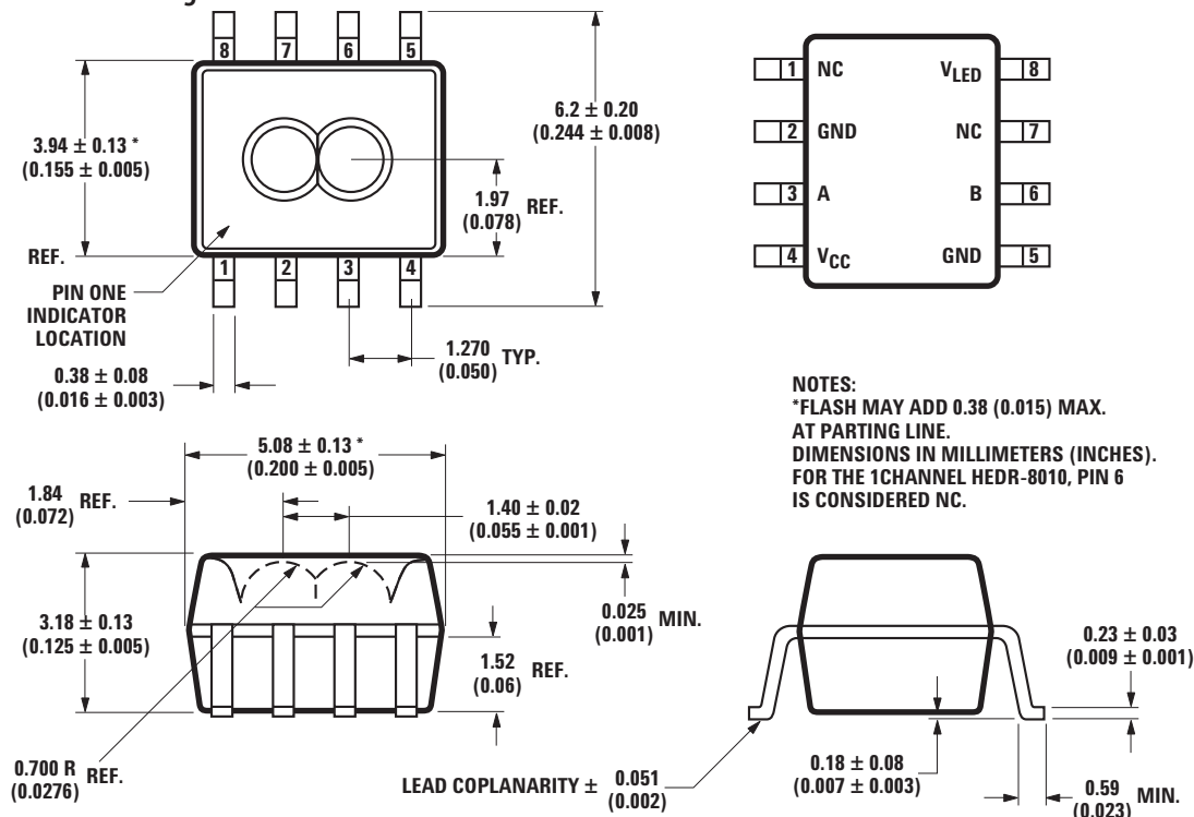
HEDR-8000 outline drwg
