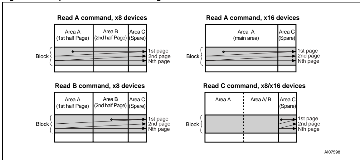
Figure 12. Read block diagrams
