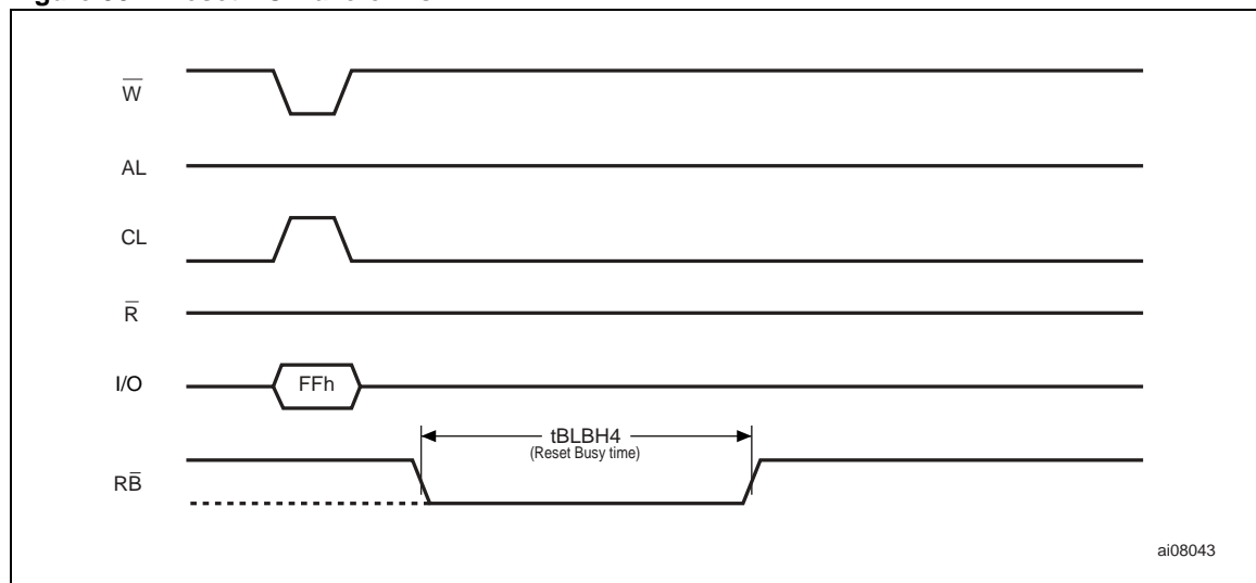
Figure 30. Reset AC waveforms
