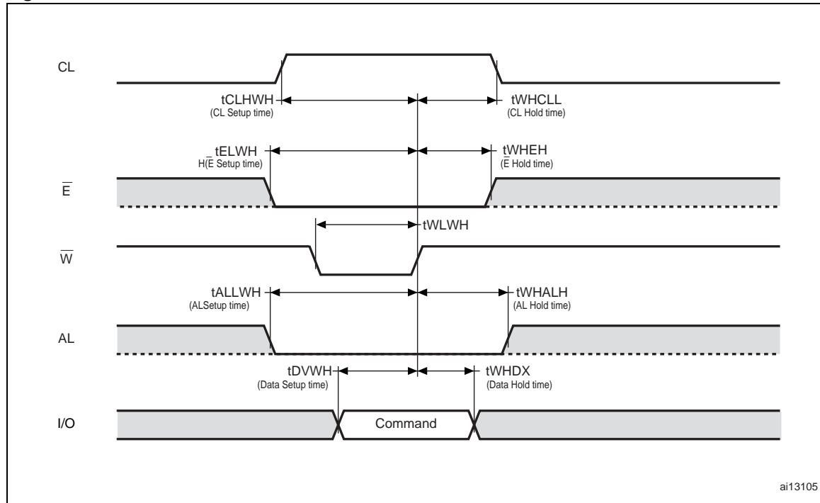
Figure 20. Command Latch AC waveforms
