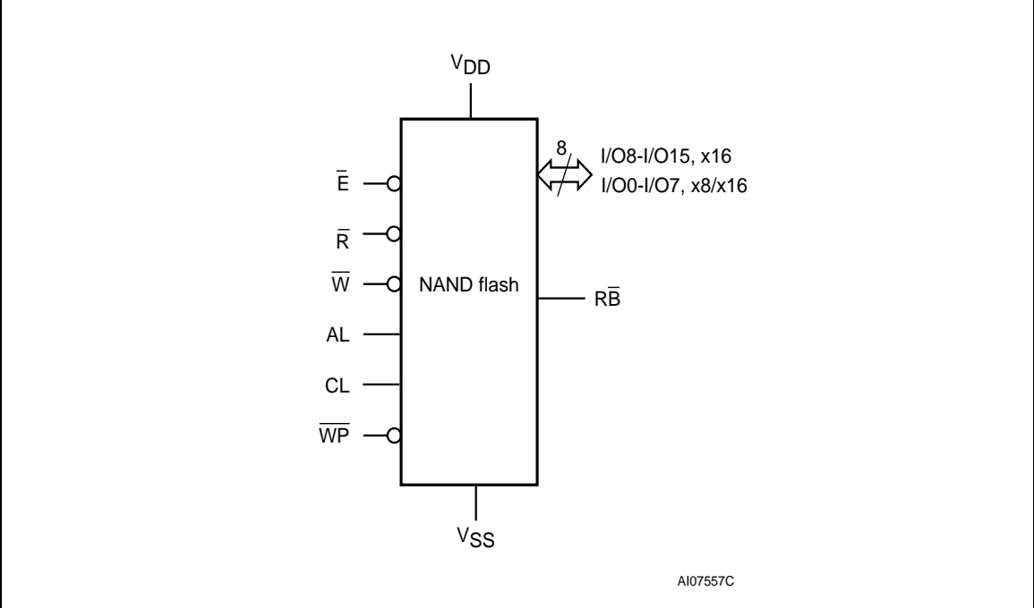
Figure 1. Logic diagram
