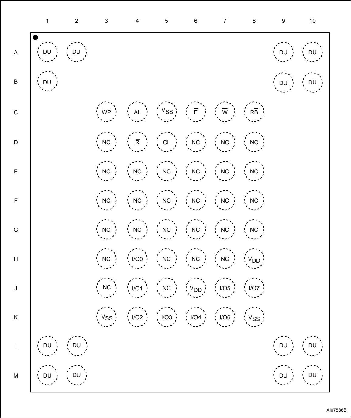
Figure 5. VFBGA63 connections - x8 devices (top view through package)
