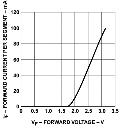
Figure 6. Forward current vs. forward voltage.
