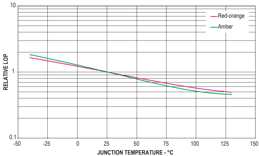
Figure 7. Relative light output vs. junction temperature
