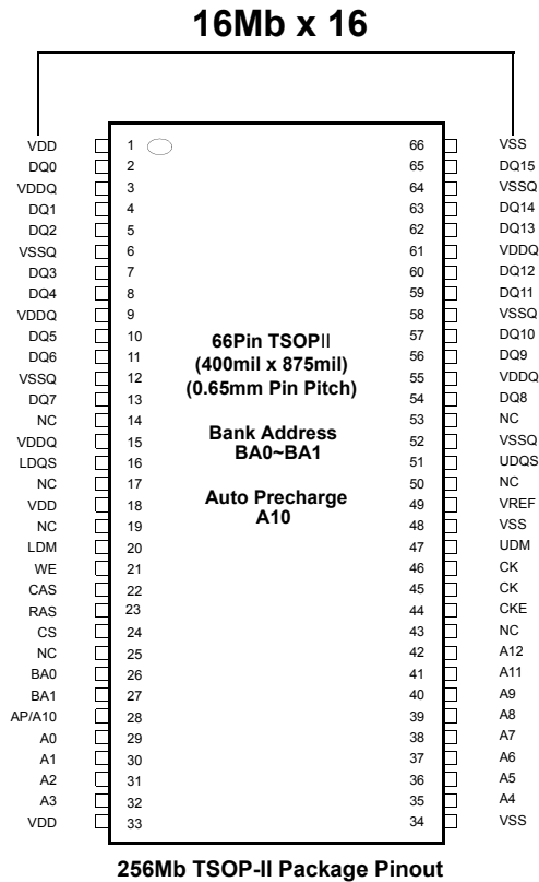
256Mb TSOP-II Package Pinout
