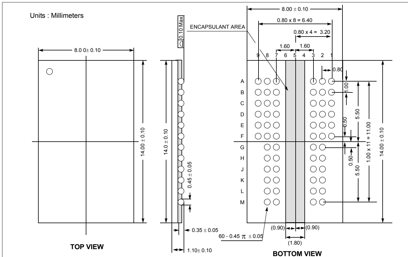
60Ball FBGA Package Dimension
