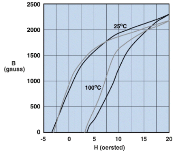
Measured on a 19/10/6mm toroid at 10 kHz.
