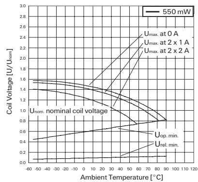
Coil operative range graphs
