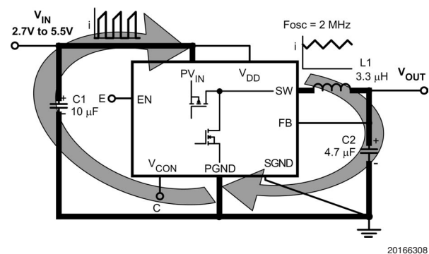
FIGURE 4. Current Loop
