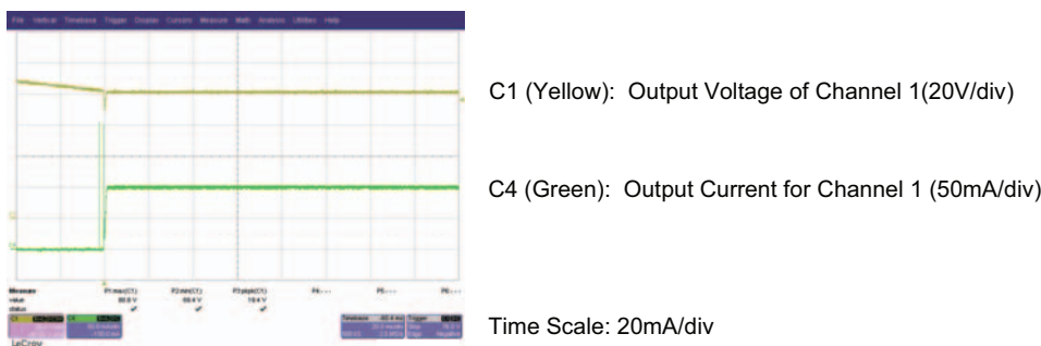
Fig. 5: Recovery from Open LED Operation
