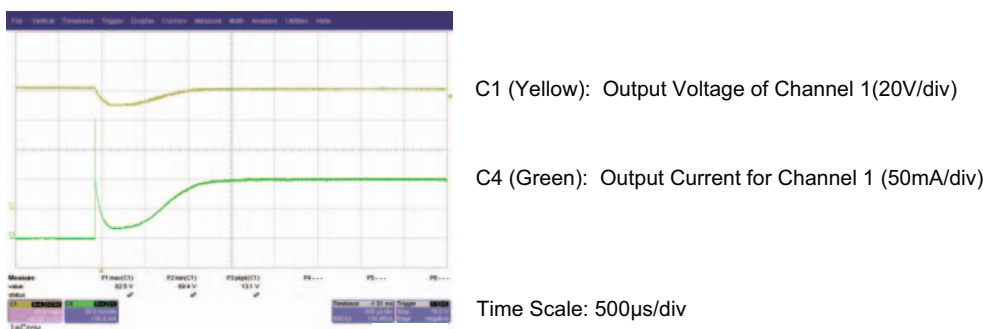
Fig. 6: Recovery (smaller timescale)
