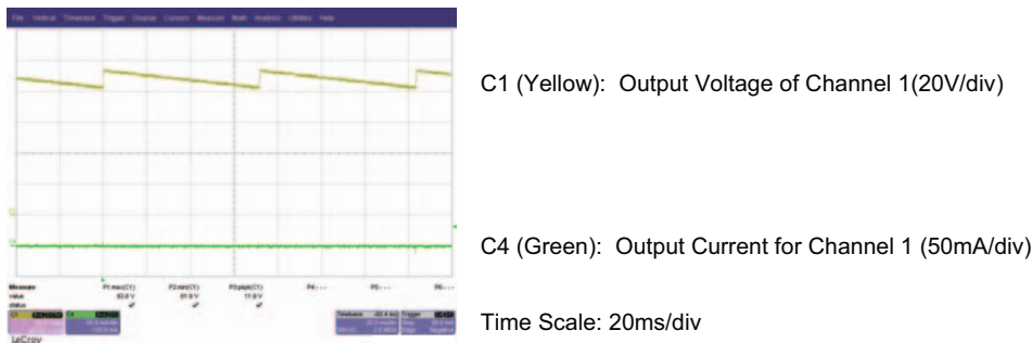
Fig. 4: Open LED Operation
