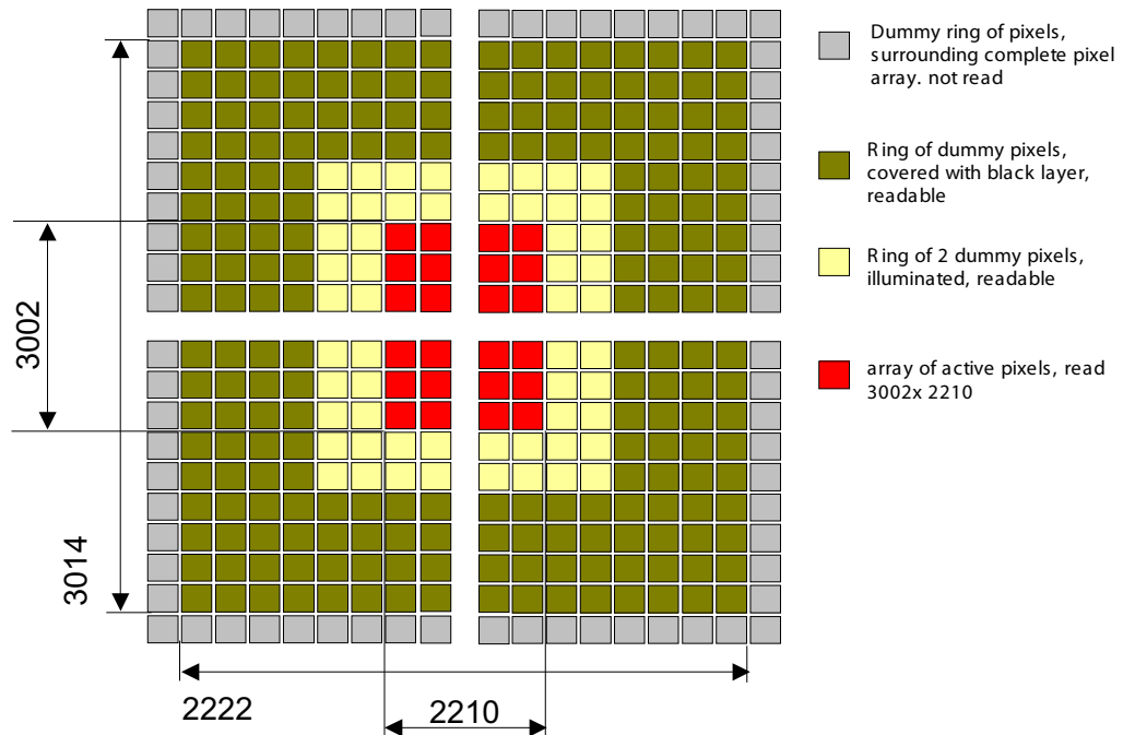
Figure 6. Floor Plan Pixel Array
