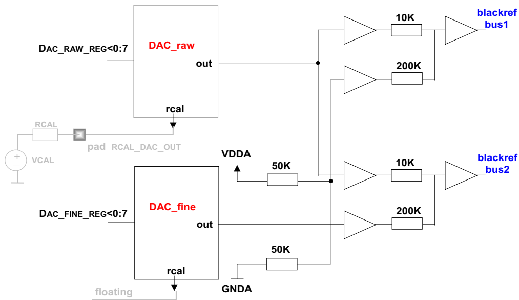
Figure 8. Offset for the Two Channels through DAC_RAW and DAC_FINE
