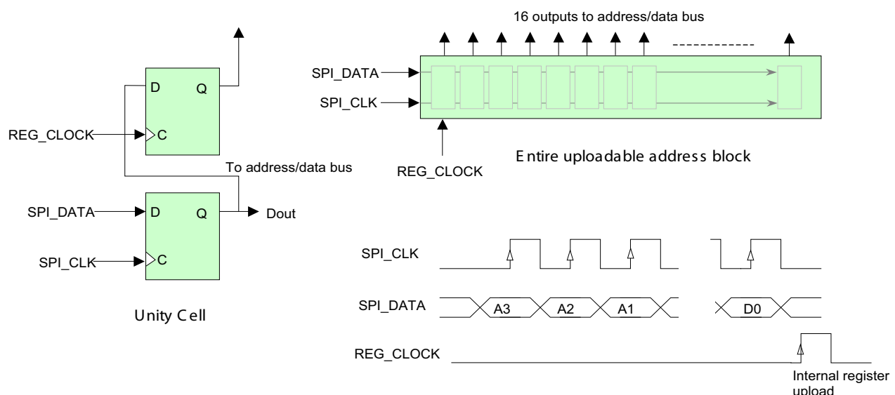
Figure 9. SPI Interface
