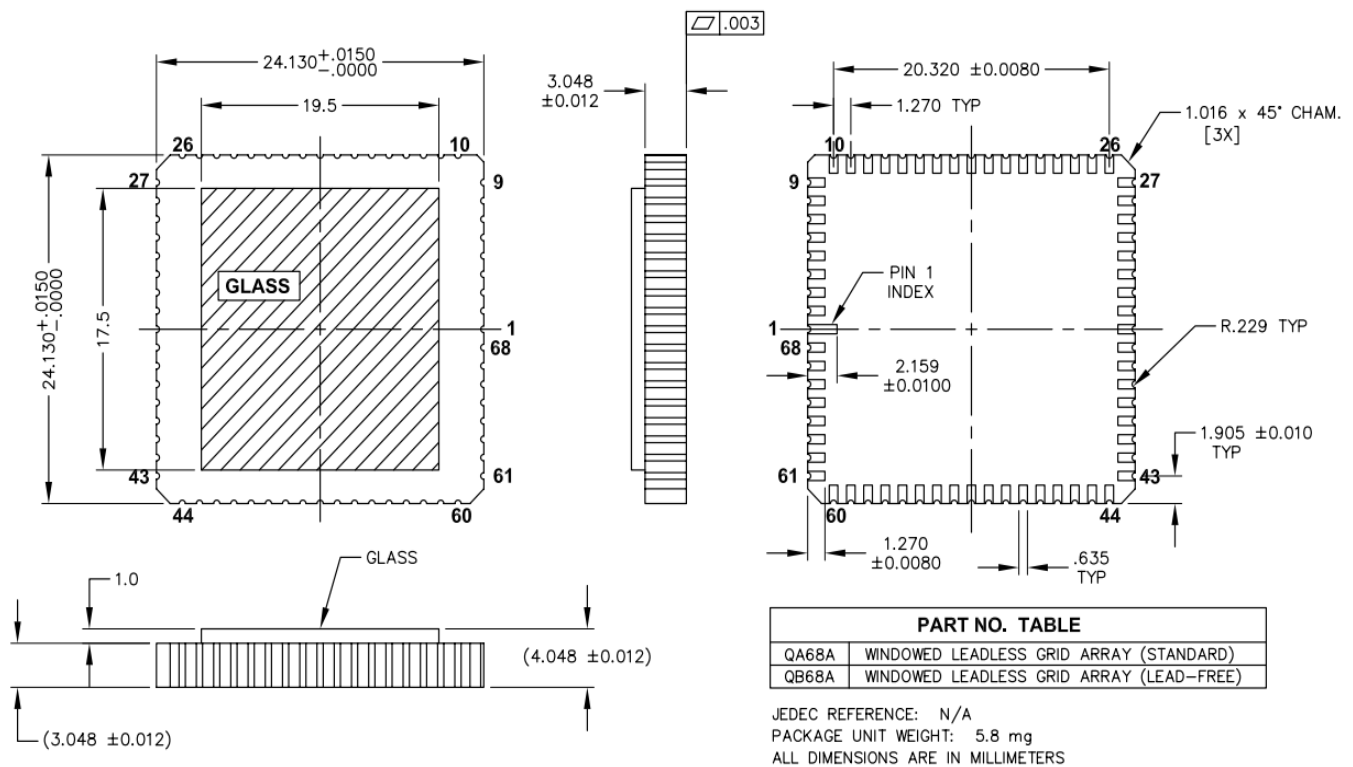
Figure 23. 68 Pin LCC Packaging Outline
