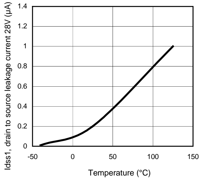
Figure 10 – Idss1 (µA) Vs temperature (°C)
