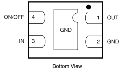
Figure 3 - TDFN4 1.2 mm x 1.6 mm Package
