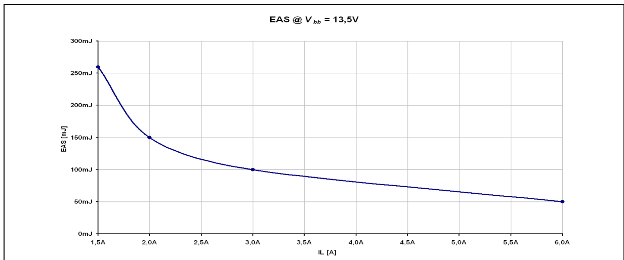
Figure 9 Maximum Energy Dissipation Single Pulse, T_{j,Start} = 150^\circ\text{C}
