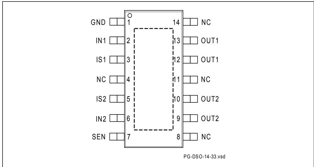
Figure 3 Pin Configuration PG-DSO-14-33
