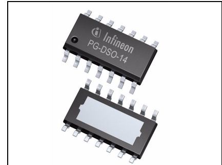
PG-DSO-14-33
