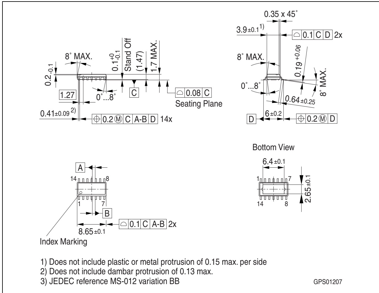
Figure 19 PG-DSO-14-33 (Plastic Dual Small Outline Package)
