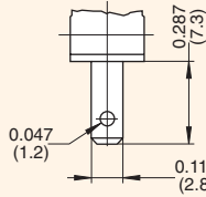
PCB Terminals – Straight 0.024 x 0.020 (0.6 x 0.5)
