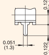
PCB Terminals LH Side w/o Location Pins 0.024 x 0.020 (0.6 x 0.5)
