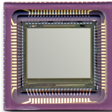
Figure 1. IBIS5-1300 Photo
