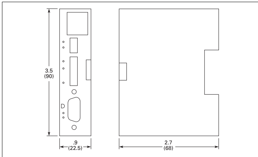
Figure 73. D77D-EMA — Approximate Dimensions in Inches (mm)
