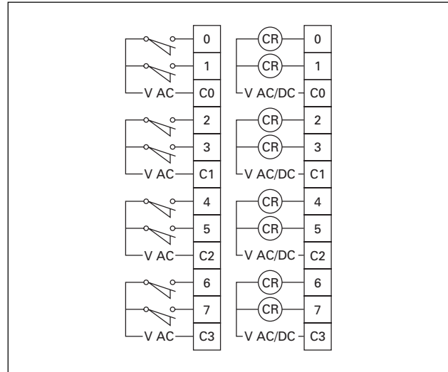
Figure 58. Wiring Diagram — AC Input Relay Output
