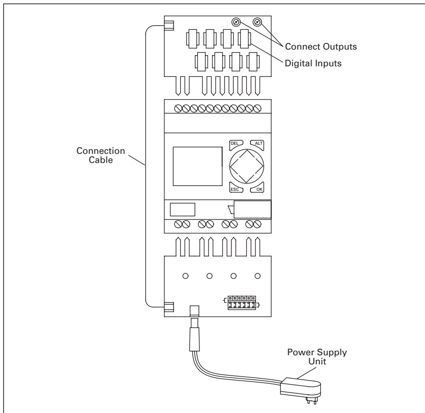
Figure 38. EZ412-DC-SIM-NA Series
