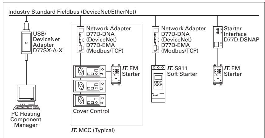
Figure 79. Network Diagram
