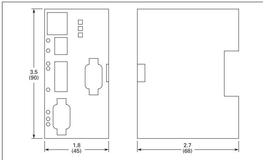
Figure 77. D77D-PNA — Approximate Dimensions in Inches (mm)
