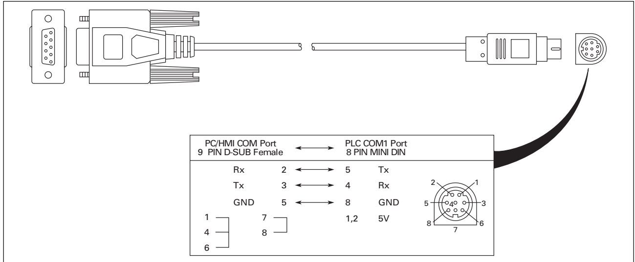
Figure 6. ELC-CBPCELC3 Cable
