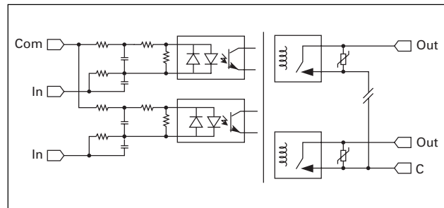
Figure 59. Circuit Diagram — AC Input Relay Output
