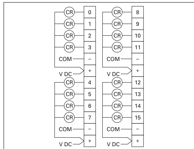
Figure 50. Wiring Diagram — DC Output Modules, D77A-DQ8 & D77A-DQ16
