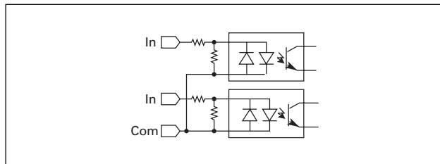
Figure 49. Circuit Diagram — DC Input Modules, D77A-DI8 & D77A-DI16
