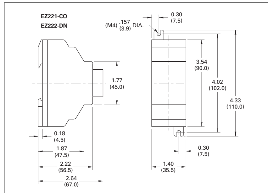
Figure 27. EZ221-CO/EZ222-DN Series Dimensions in Inches (mm), Drawing Number MD05013010E
