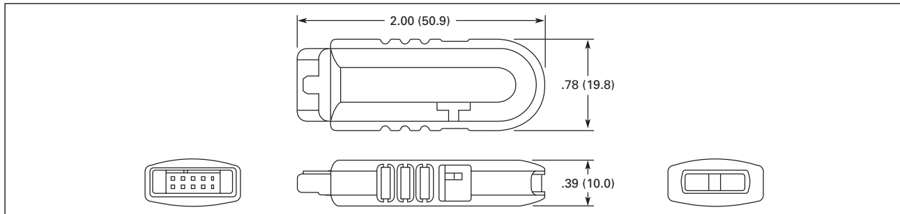
Figure 12. ELC-GPXFERMOD — Approximate Dimensions in Inches (mm)
