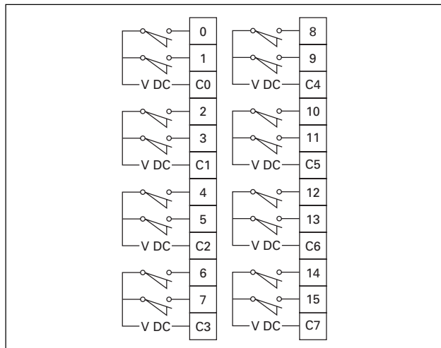
Figure 48. Wiring Diagram — DC Input Modules, D77A-DI8 & D77A-DI16
