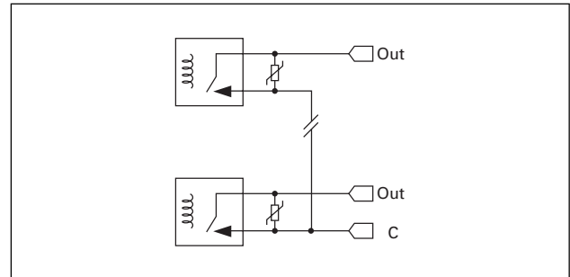
Figure 53. Circuit Diagram
