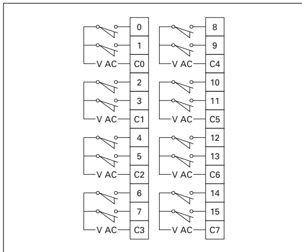
Figure 44. Wiring Diagram — AC Input Modules, D77A-AI8 & D77A-AI16
