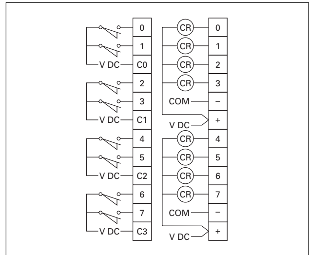
Figure 56. Wiring Diagram — DC Input DC Output
