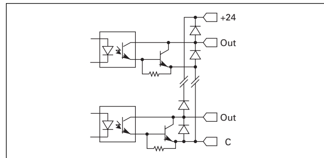
Figure 51. Circuit Diagram — DC Output Modules, D77A-DQ8 & D77A-DQ16
