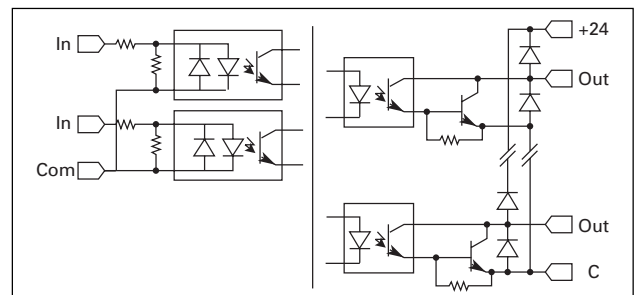
Figure 57. Circuit Diagram — DC Input DC Output
