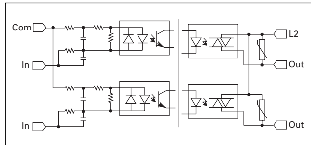
Figure 55. Circuit Diagram — AC Input AC Output
