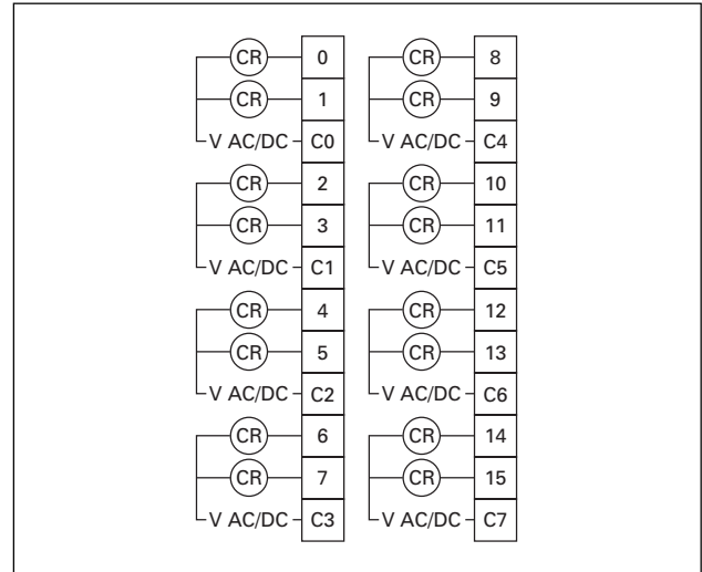
Figure 52. Wiring Diagram
