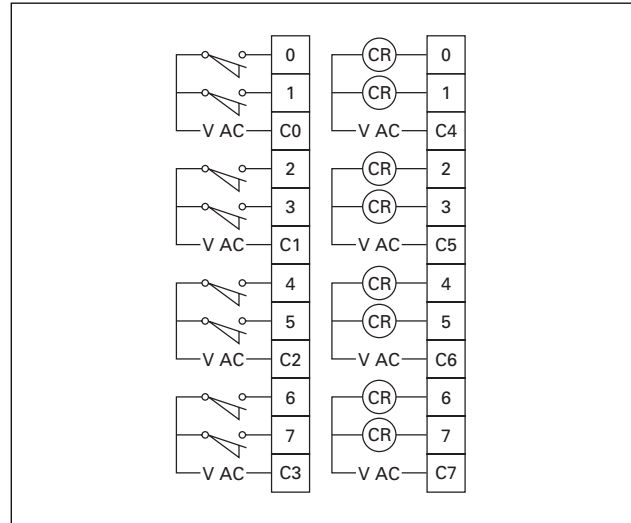
Figure 54. Wiring Diagram — AC Input AC Output
