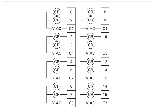
Figure 46. Wiring Diagram — AC Output Modules, D77A-AQ8 & D77A-AQ16
