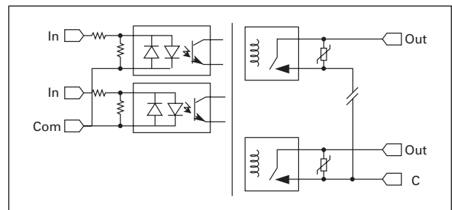
Figure 61. Circuit Diagram — DC Input Relay Output
