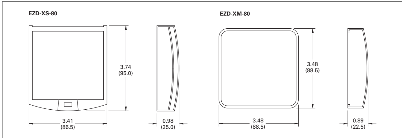
Figure 32. EZD-XS-80 and EZD-XM-80 Series Dimensions in Inches (mm), Drawing Number MD05013009E
