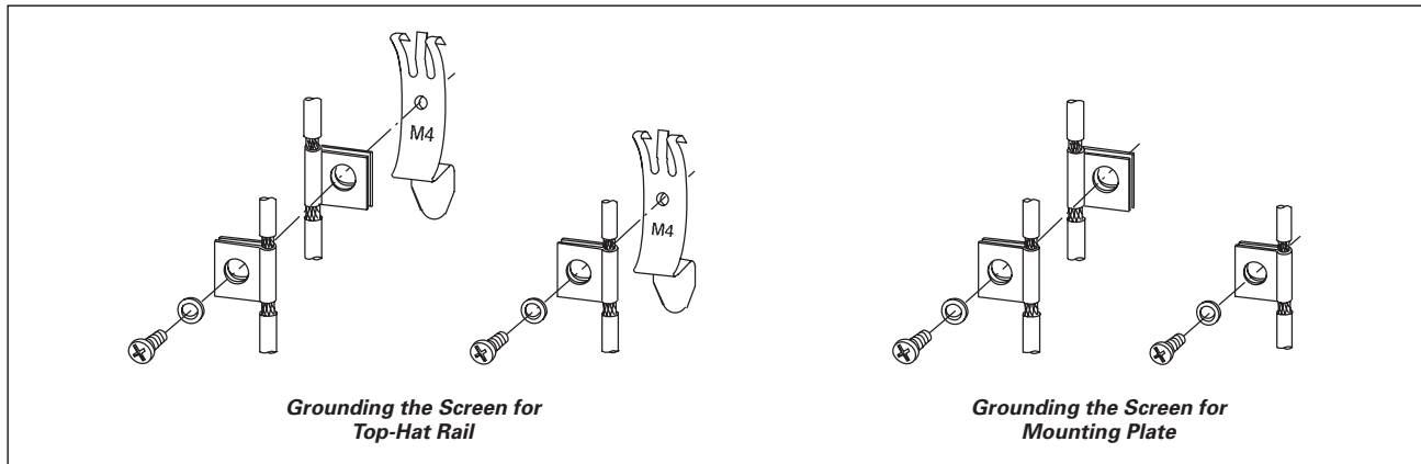
Figure 37. EZB4-102-KS1 Series
