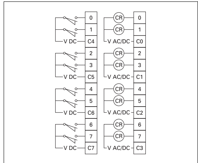
Figure 60. Wiring Diagram — DC Input Relay Output
