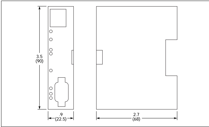
Figure 75. D77D-EIP — Approximate Dimensions in Inches (mm)
