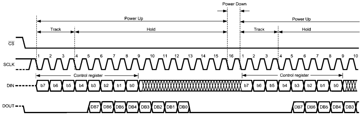
ADC082S051 Operational Timing Diagram
