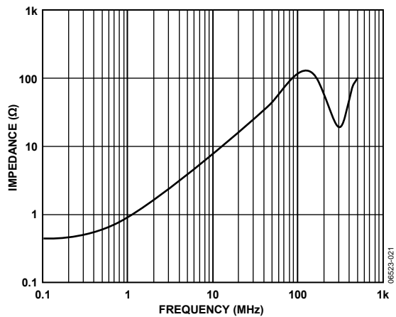
Figure 26. Enabled Output Impedance vs. Frequency, V_S = \pm 5 V
