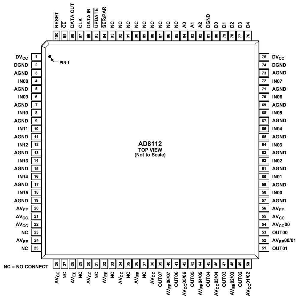
Figure 6. Pin Configuration
