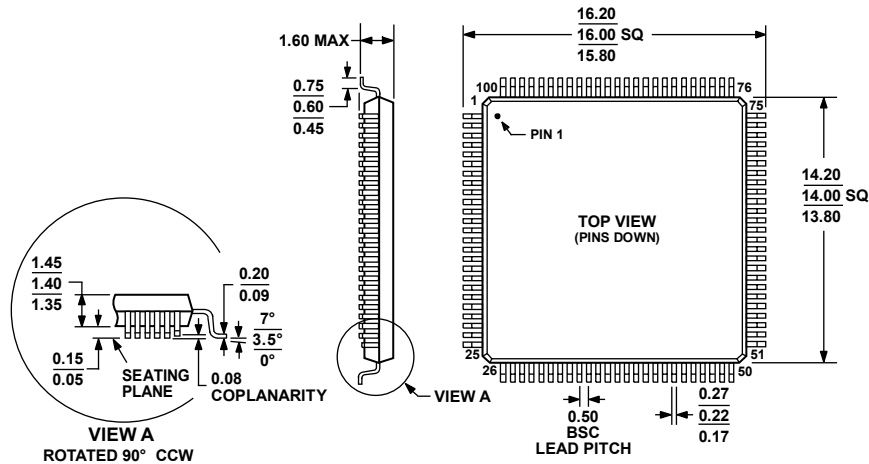
COMPLIANT TO JEDEC STANDARDS MS-026-BED Figure 49. 100-Lead Low Profile Quad Flat Package [LQFP] (ST-100) Dimensions shown in millimeters
