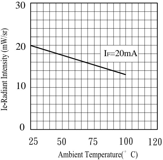
Fig.7 Radiant Intensity vs. Ambient Temperature(°C)
