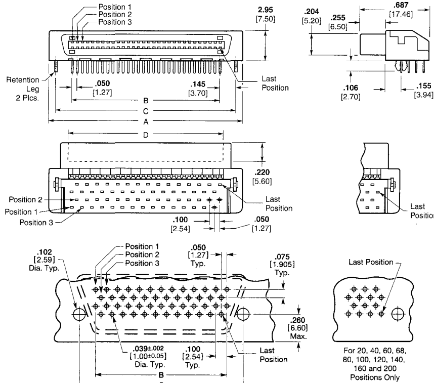
Recommended PC Board Layout Component Side For 30, 50 and 130 Positions Only
