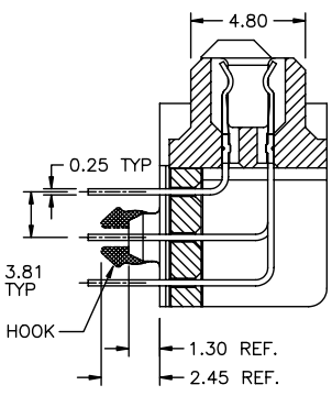
SECTION X-X 4/1
