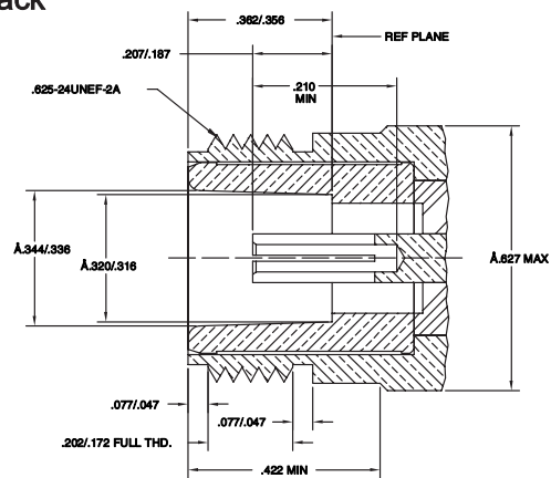
Jack
