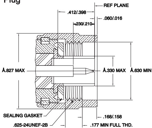
Plug
