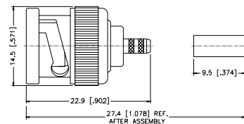
Assembly Instruction J - page 236
