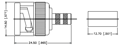
Assembly Instruction J - page 236
