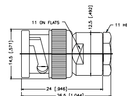
Assembly Instruction P - page 242
