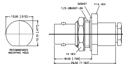
Assembly Instruction N - page 240
