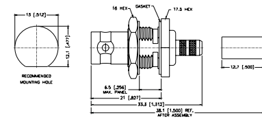
Assembly Instruction J - page 236
