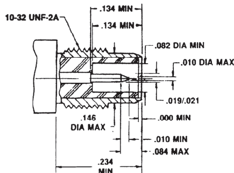
Plug
