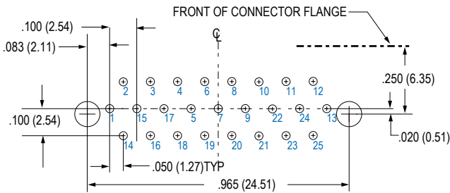
25 PIN MWDM-25PCBR
