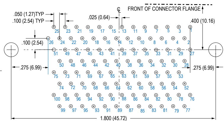
100 SOCKET MWDM-100SCBR
