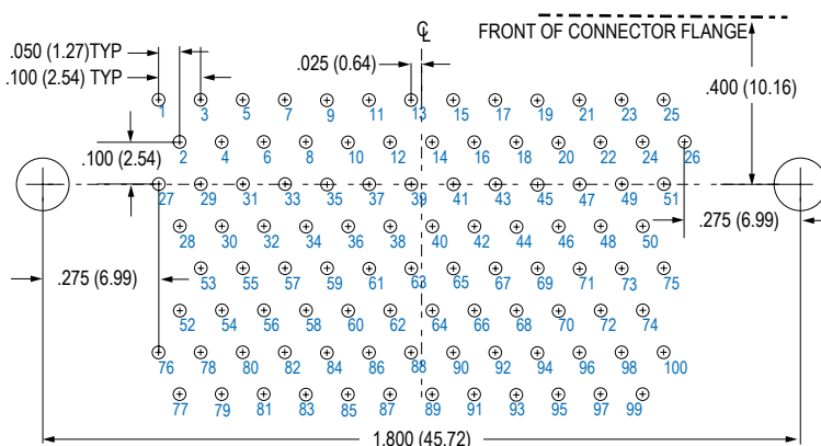
100 PIN MWDM-100PCBR
