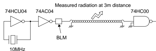
Testing Circuit
