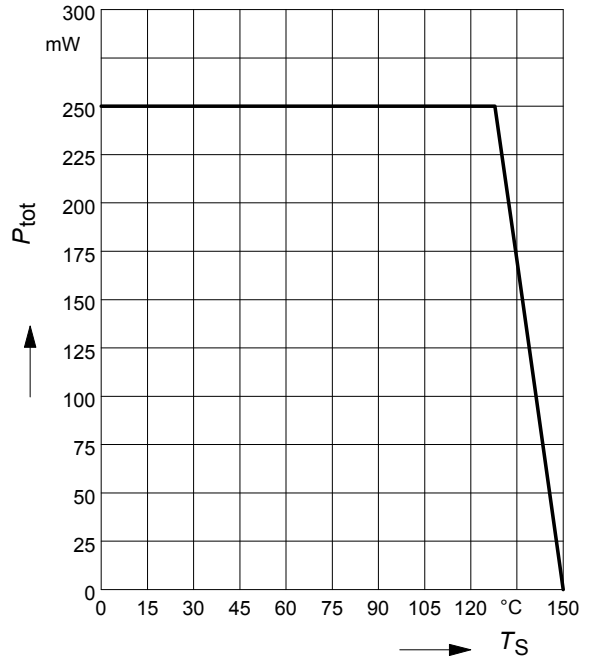
Total power dissipation P_{tot} = f(T_S) BCR129W
