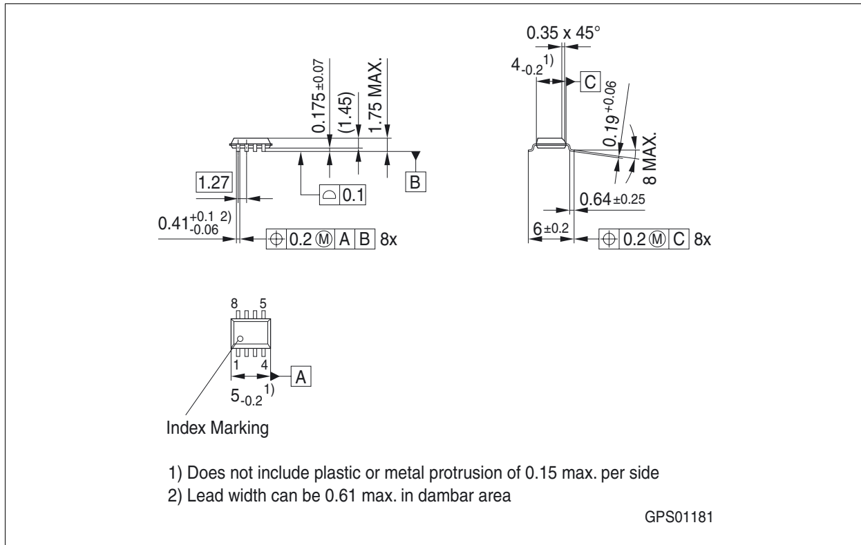
Figure 1 PG-DSO-8-25
